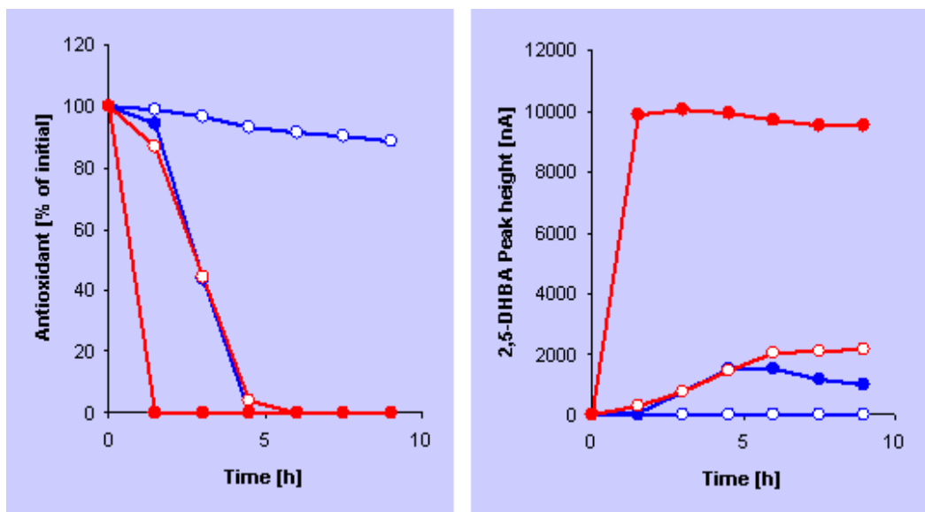
Figure 5: Incubation of salicylate with 500 \mu\text{M} NADH (blue) or ascorbate (red) in the absence (open symbols) or presence (full symbols) of \text{Cu}^{2+} (10 \mu\text{M} ). Left: Consumption of antioxidant; Right: Formation of 2,5-dihydroxybenzoic acid (DHBA).
